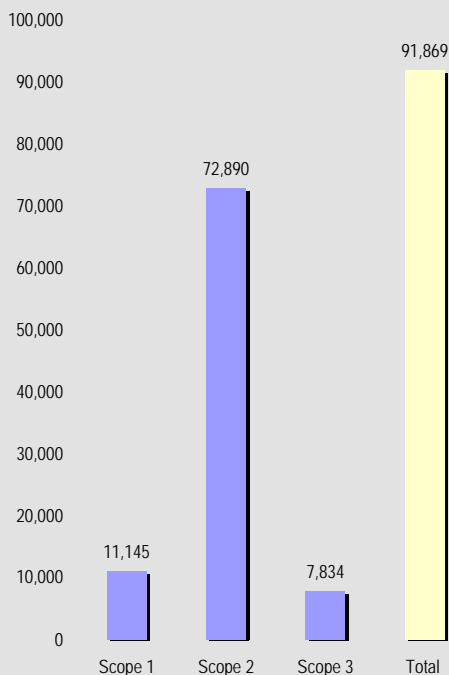
Global Metric Tonnes of CO 2 -equivalent by Scope - 2007
